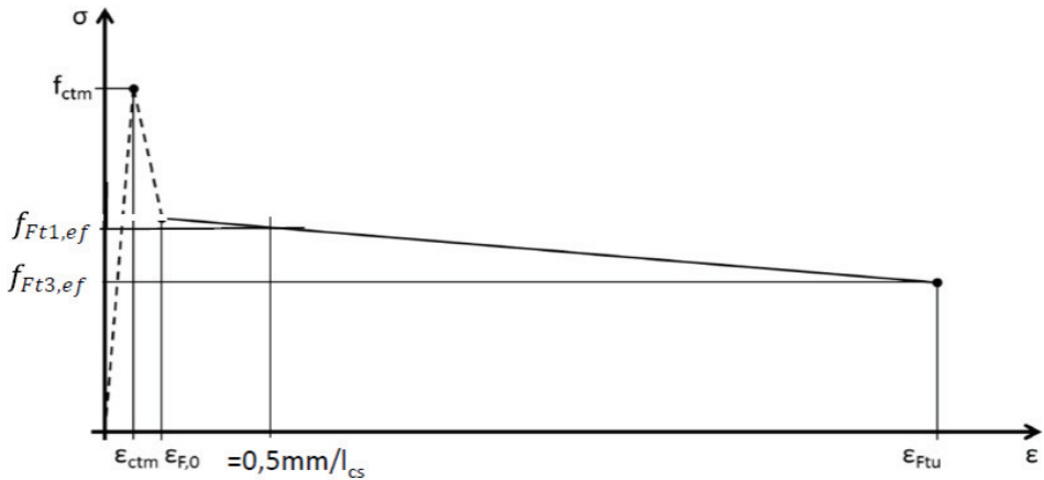
Figure C3.2. Constitutive Law
