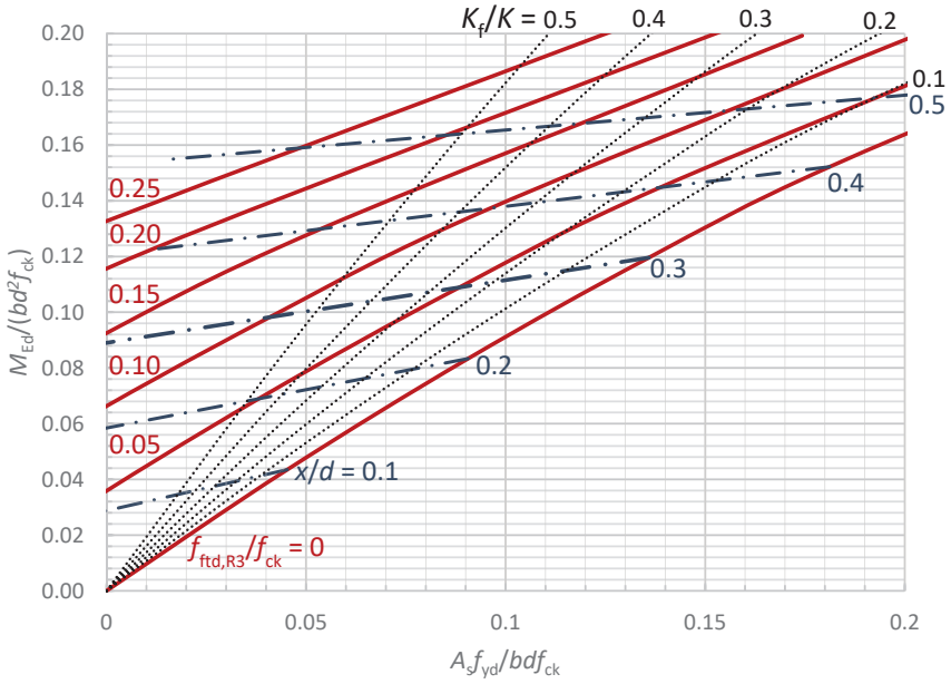
Chart A-1. ( d/h = 0.80 )
