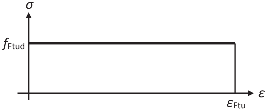
Figure C6.1. Plastic Distribution
