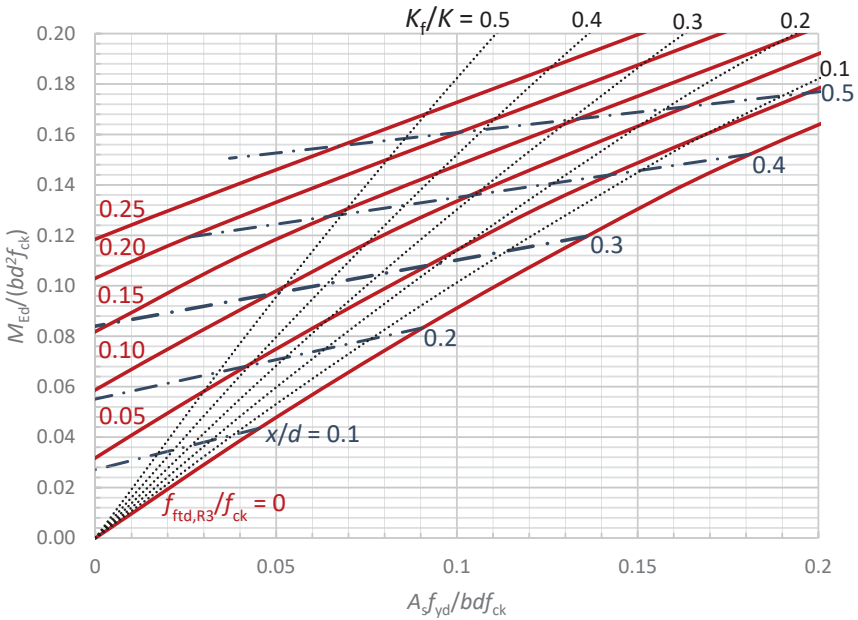
Chart A-2. ( d/h = 0.85 )
